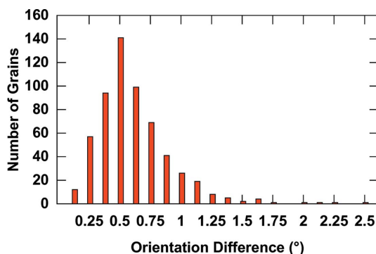
Figure 18 A histogram of disorientation angle between matched grain pairs in the DCT and TriBeam tomography data sets is shown. Most grain pairs exhibit an angle of between 0.25 and 0.75^\circ .
